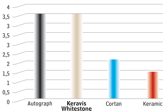
ABRASION RESISTANCE ACCORDING TO LGA TESTS
